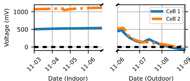
c) Open circuit voltage during the transition from lab-to-field.
