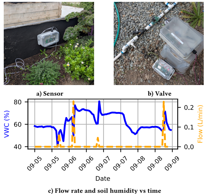
Figure 9: Beyond traditional sensing applications, ENTS is capable of extending to actuation and control. Demonstrated by drip irrigation driven and monitored by ENTS.
