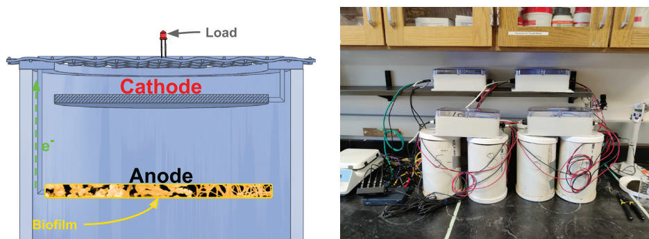
FIGURE 2. (a) Diagram of a microbial fuel cell with carbon felt electrodes. Initially there is no potential, but as a microbial biofilm forms, power output rises. (b) A photograph of cells in the laboratory. After 60 days, the biofilm is able to provide a consistent output of 15-25 \mu\text{W} .
